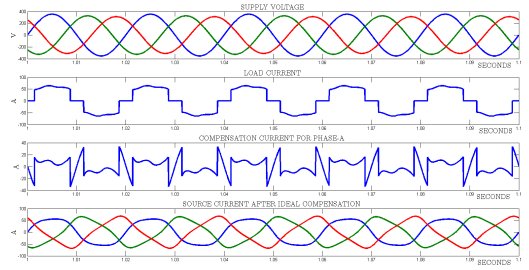
Fig. 8. Case-4: Performance of IARPT under unbalanced condition: ( V_a = 250V \angle 0^\circ ; V_b = 230V \angle -130^\circ ; V_c = 220V \angle 125^\circ )
