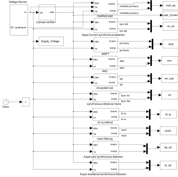
Fig. 1. Simulink model developed to compare the algorithms
